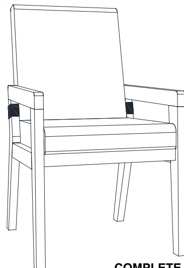
COMPLETE ASSEMBLY
